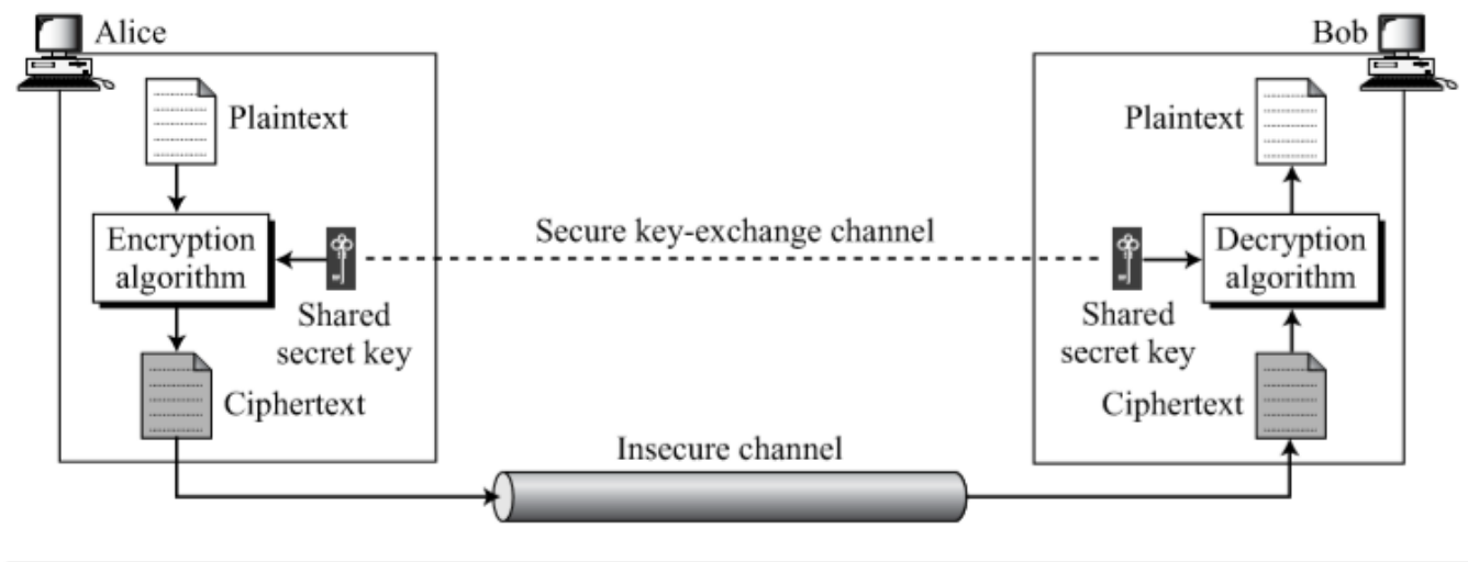
Figure 3.1 General idea of symmetric-key cipher
