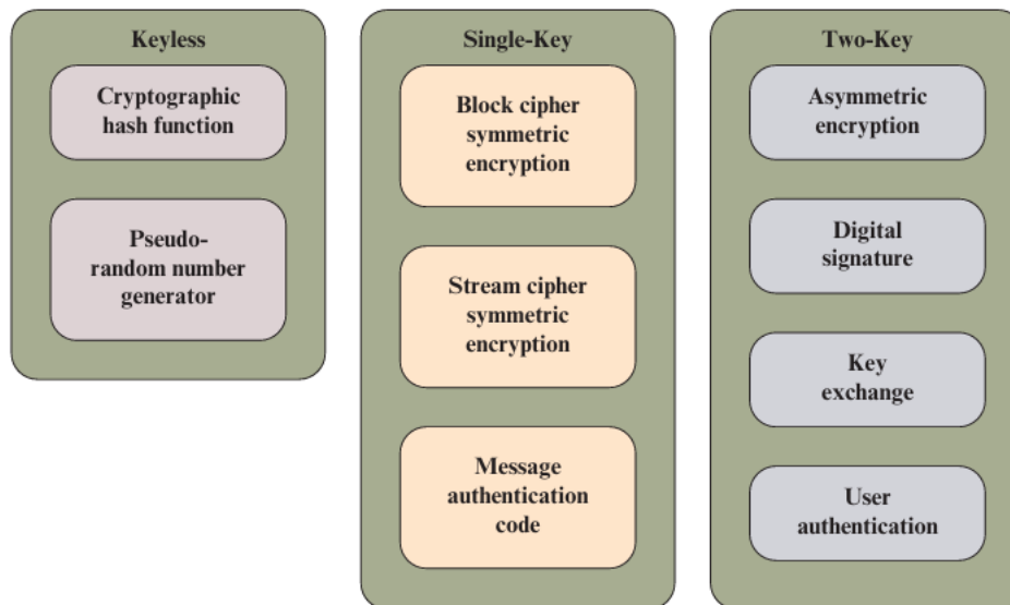
Figure 1.4 Cryptographic Algorithms
