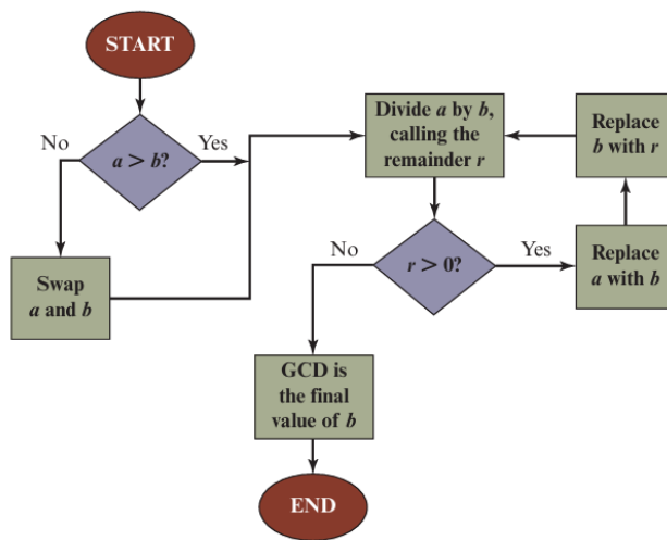
Figure 2.2 Euclidean Algorithm
